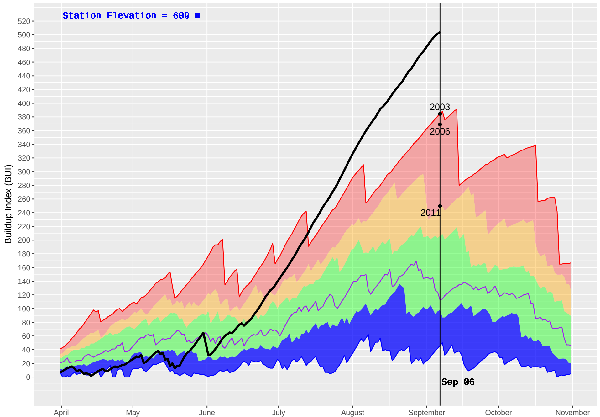
ROCK CREEK (394) : Historical (1990–2016) and Current (2017) Noon Buildup Index (BUI)
